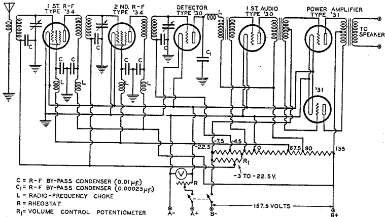
TYPICAL TUNED RADIO-FREQUENCY CIRCUIT 2-VOLT FILAMENT TYPES
