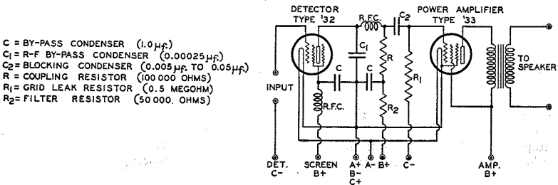
OPTIONAL DETECTOR AND AMPLIFIER—2-VOLT FILAMENT TYPES
